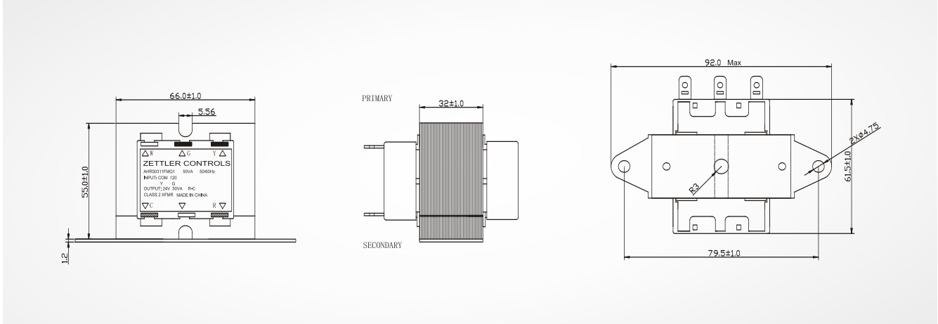
TYPE FMQ1 FOOT MOUNT ONE SIDE QD TERMINALS
