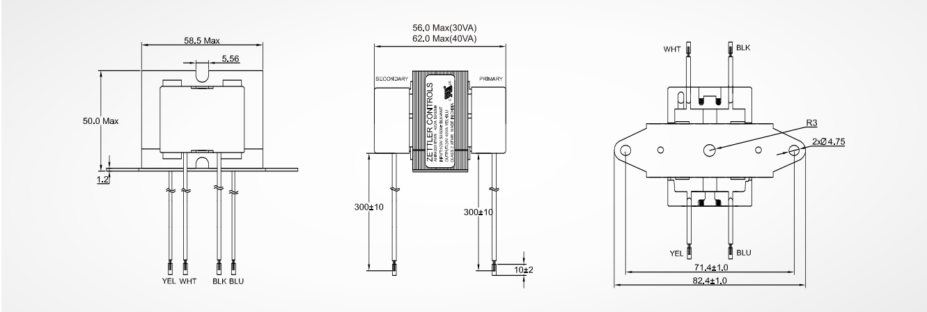
TYPE FMW FOOT MOUNT BRACKET WITH WIRE LEADS
