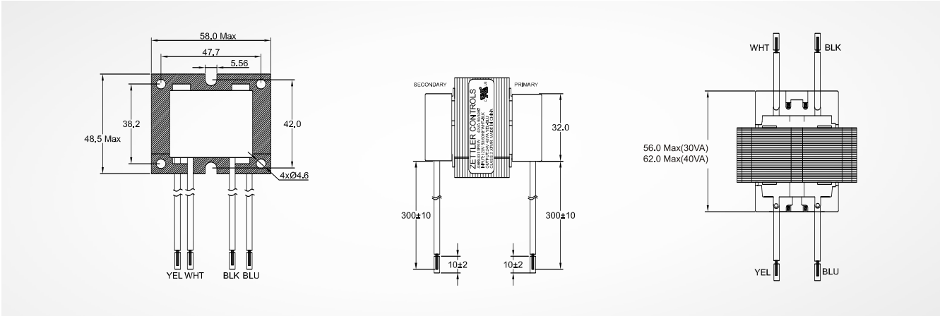
TYPE PM PANEL MOUNT
