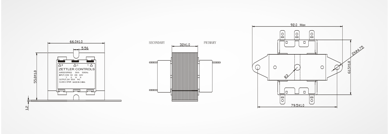
TYPE FMQ2 FOOT MOUNT BOTH SIDES QD TERMINALS
