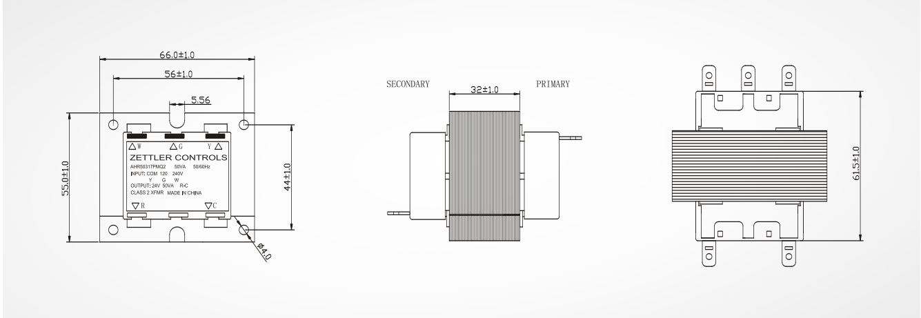
TYPE FMQT PANEL MOUNT WITH QD TERMINALS
