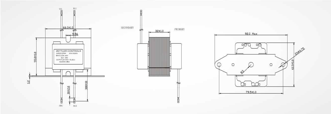
TYPE FMW FOOT MOUNT BRACKET WITH WIRE LEADS
