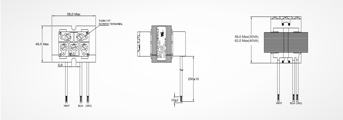
TYPE FC SCREW TERMINATION
